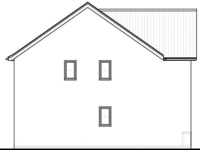
SIDE ELEVATION
